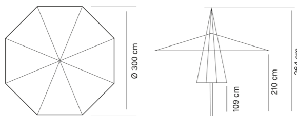
REF. 876 HEAVY DUTY Ø3 m
